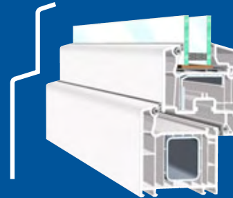
SOFTLINE 70 AD
